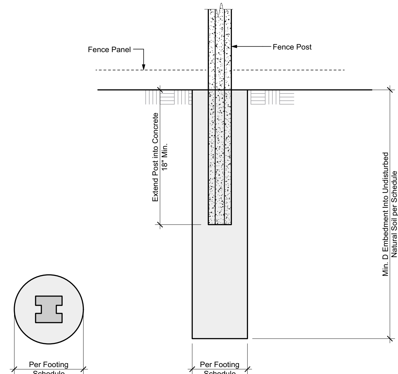
FENCE FOUNDATION SUPPORT
