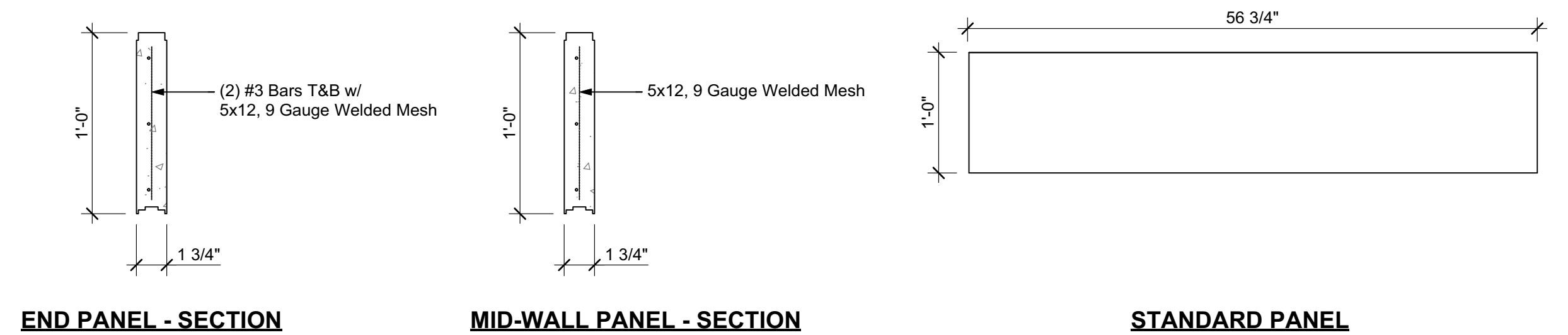
END PANEL - SECTION MID-WALL PANEL - SECTION STANDARD PANEL
