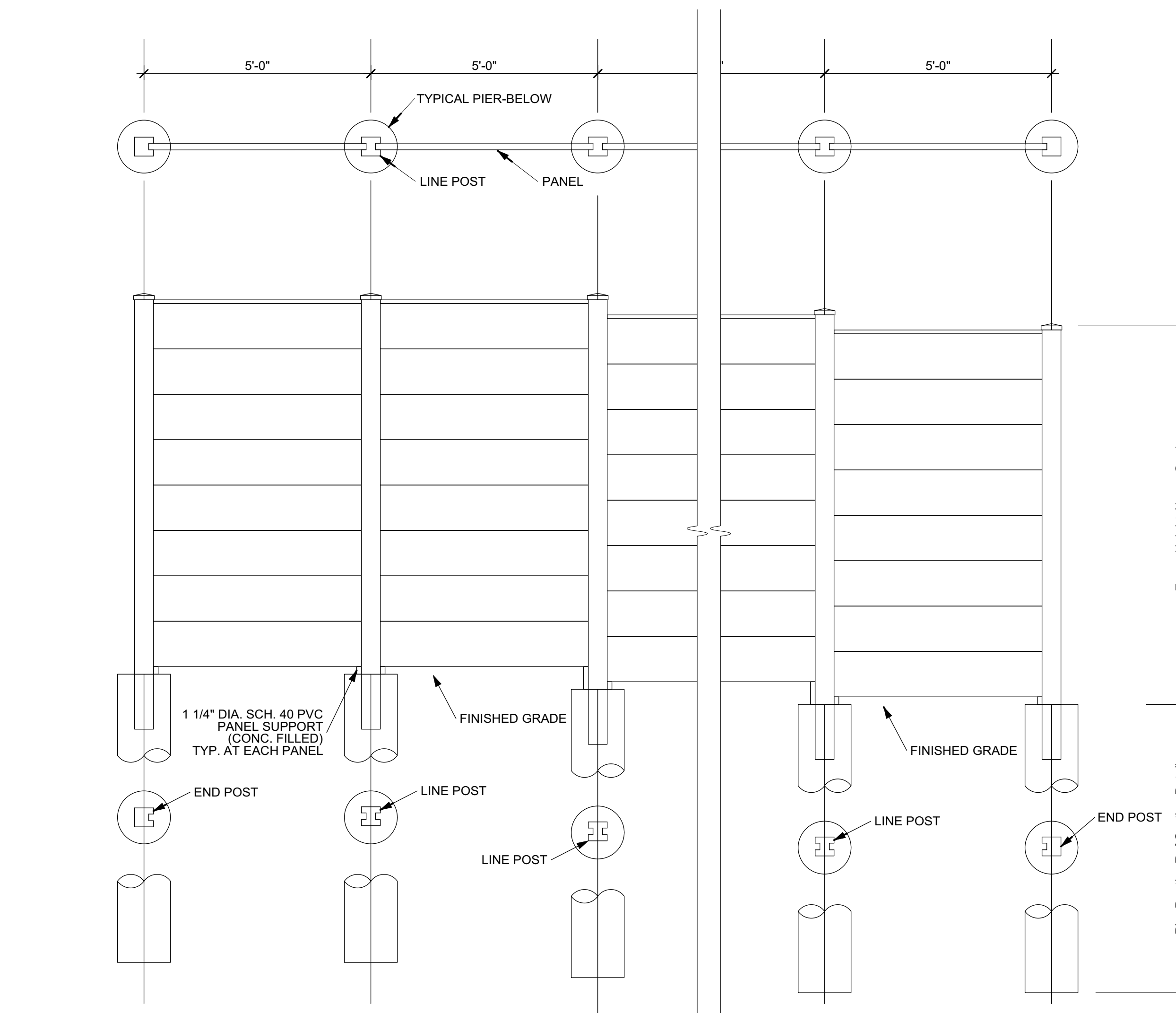
ELEVATION - SCREENING WALL AND PIERS
